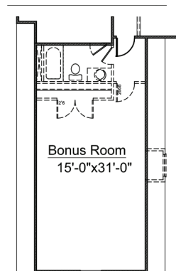
Second Floor Opt. Bonus Room #1
